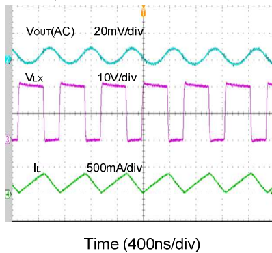
Output Ripple
