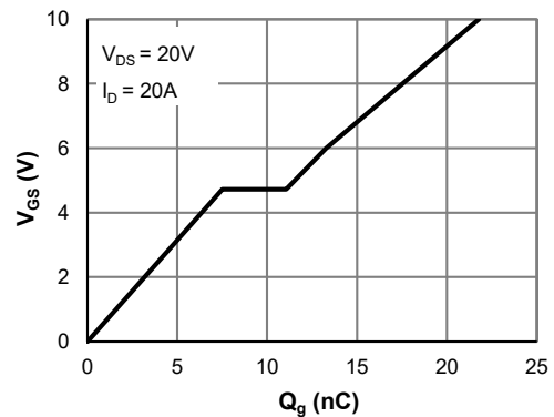
Gate Charge
