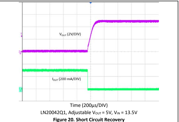
Figure 20. Short Circuit Recovery
