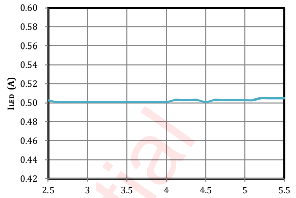
I LED =0.502A f sw =2MHz Flash LED Flash Current vs Input Voltage
