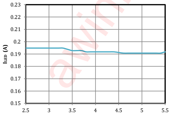
I LED =0.192A f sw =2MHz Torch LED1/2 Torch Current vs Input Voltage
