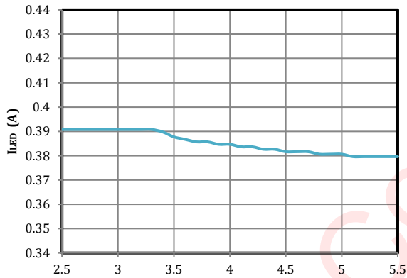
I LED =0.386A f sw =2MHz Torch LED1/2 Torch Current vs Input Voltage
