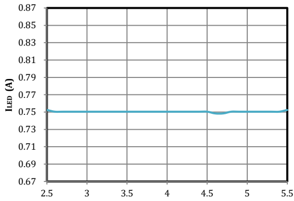
I LED =0.749A f sw =2MHz Flash LED Flash Current vs Input Voltage
