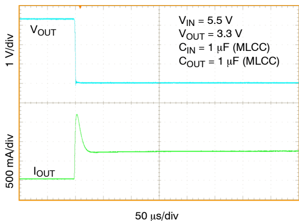
Figure 62. Short-Circuit Current Peak
