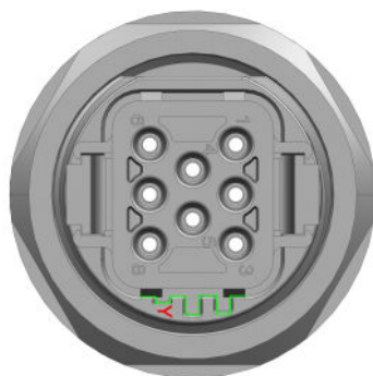
Y-Keying*
