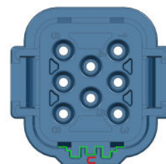
U-Keying*
