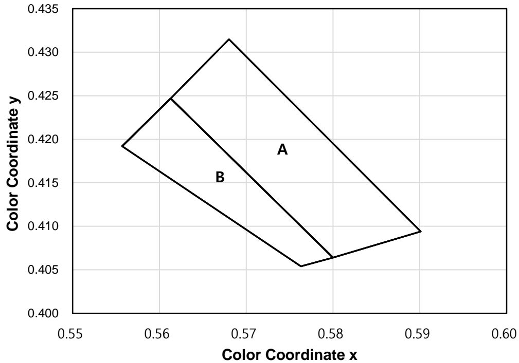
Fig 10-2. Color Coordinate Diagram of amber color, T_a = 25^\circ\text{C} , I_F = 0.35\text{A}
