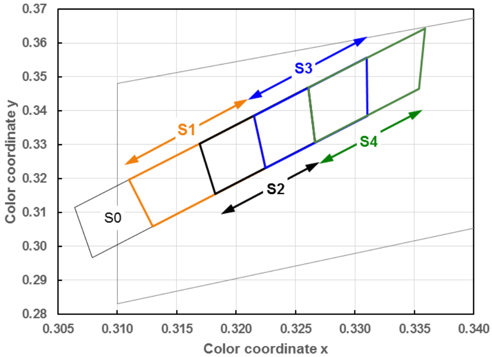
Fig 10-1. Color Coordinate Diagram of white color, T_a = 25^\circ\text{C} , I_f = 0.35\text{A}
