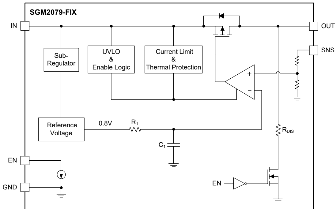
Figure 3. Fixed Output Voltage Internal Block Diagram
