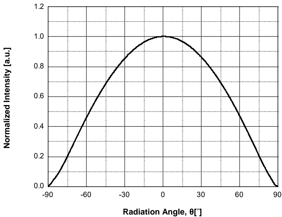
Fig 2. Viewing Angle Distribution, I_F = 50\text{mA}
