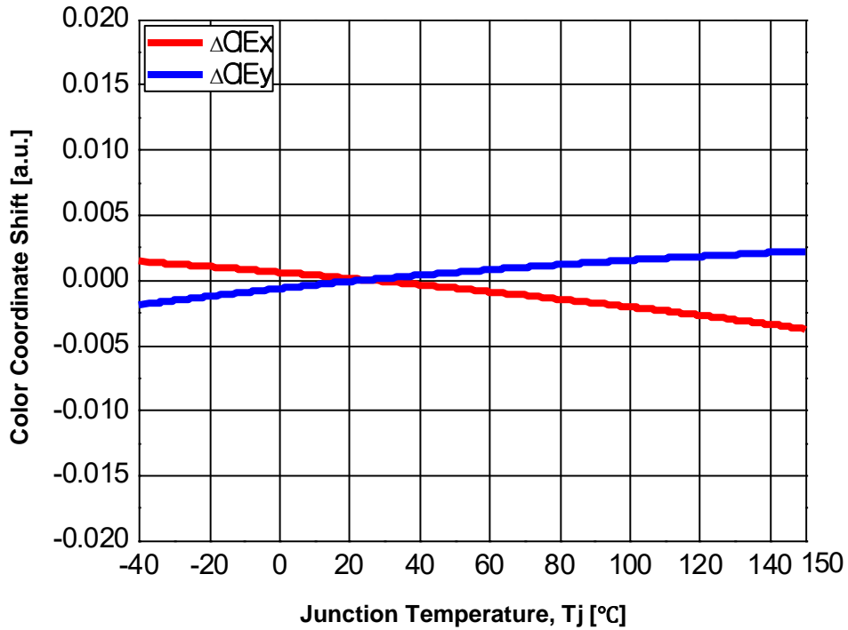
Fig 8. Junction Temperature vs. Color Coordinate Shift, I_f = 50\text{mA}
