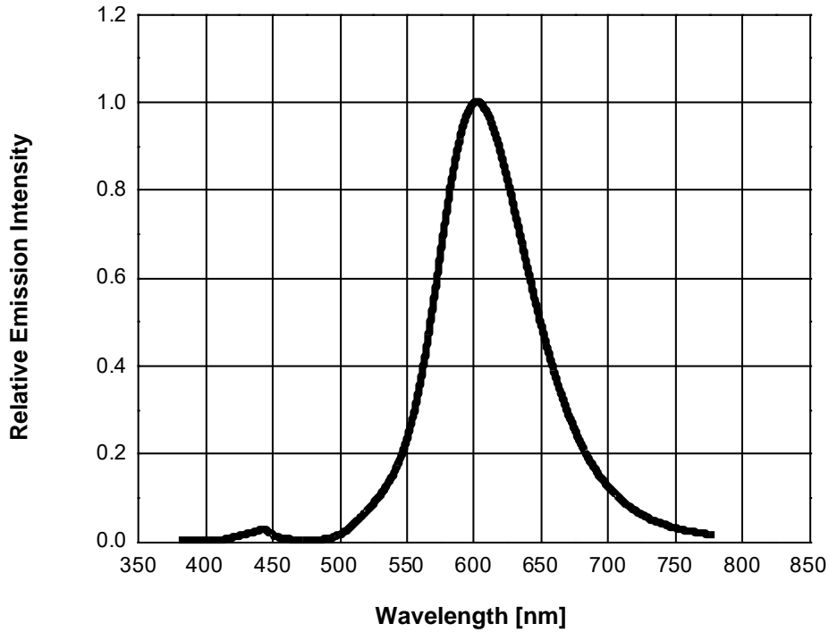
Fig 1. Color Spectrum, I_F = 50\text{mA} , T_a = 25^\circ\text{C}
