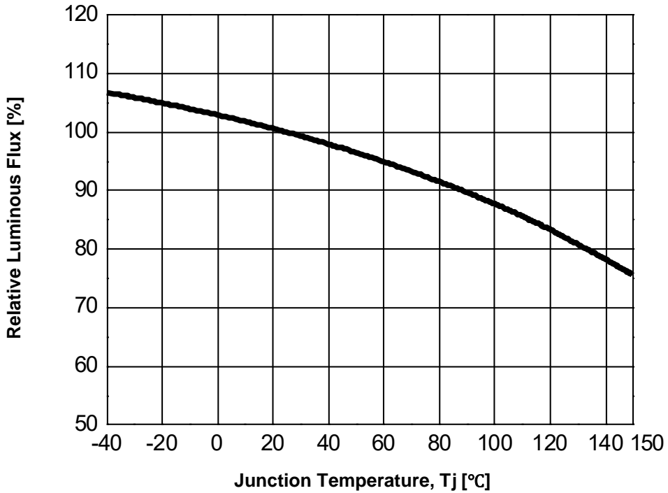
Fig 6. Junction Temperature vs. Relative Luminous Flux, I_F = 50\text{mA}
