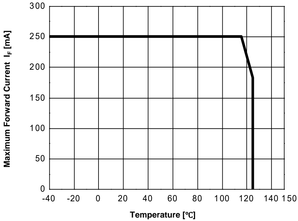
Fig 9. Maximum Allowable Forward Current vs Solder Temperature
