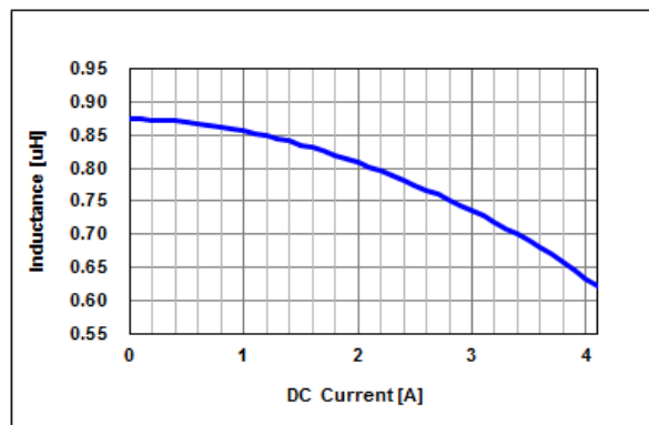
[Ex: Inductor Saturation Characteristics]
