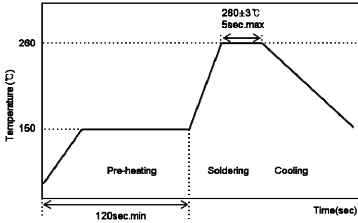
[Flow Soldering Conditions]
