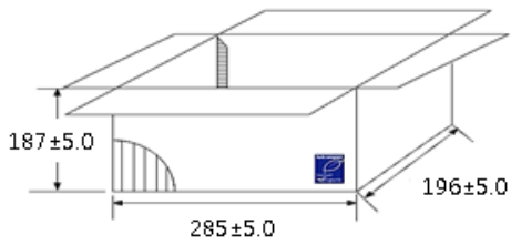
- Out Box (7" x 20 REEL)
