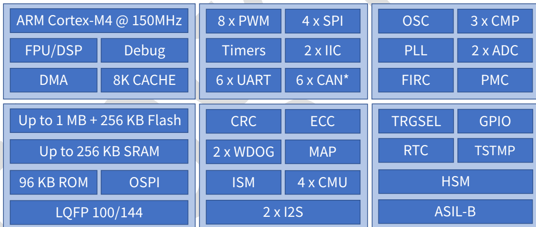
Figure 3. FC4150F1M_A block diagram
