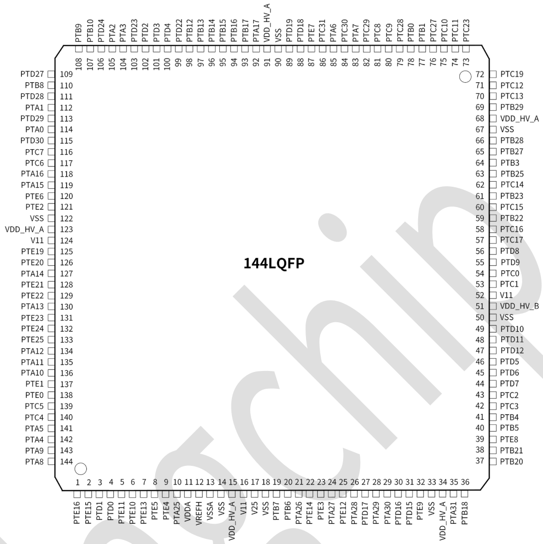
Figure 29. 144LQFP pinout
