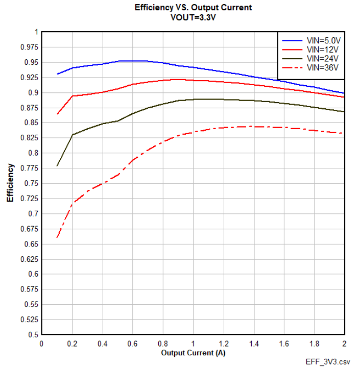
Figure 2. V OUT =3.3V, Efficiency, L=3.3 uH,LP6432H
