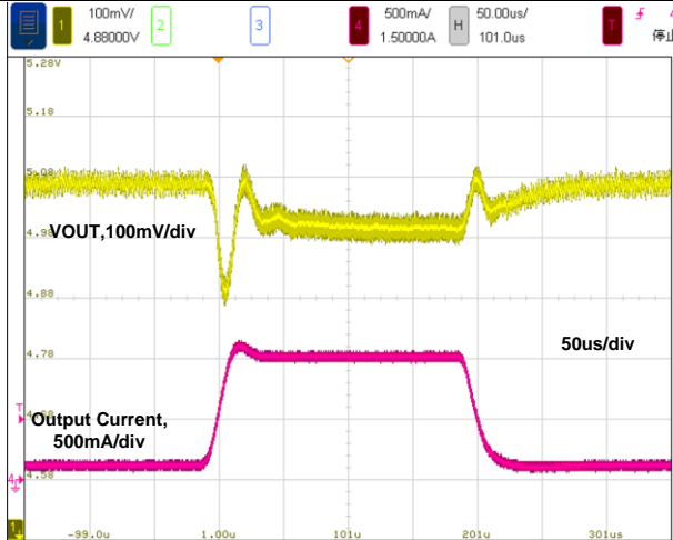
Figure 25. Load Transient, 0.1A-1A-0.1A
