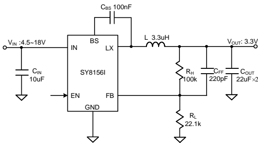
Figure1. Schematic Diagram
