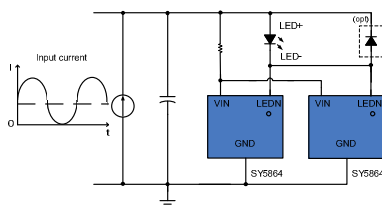
Fig. Parallel circuit
