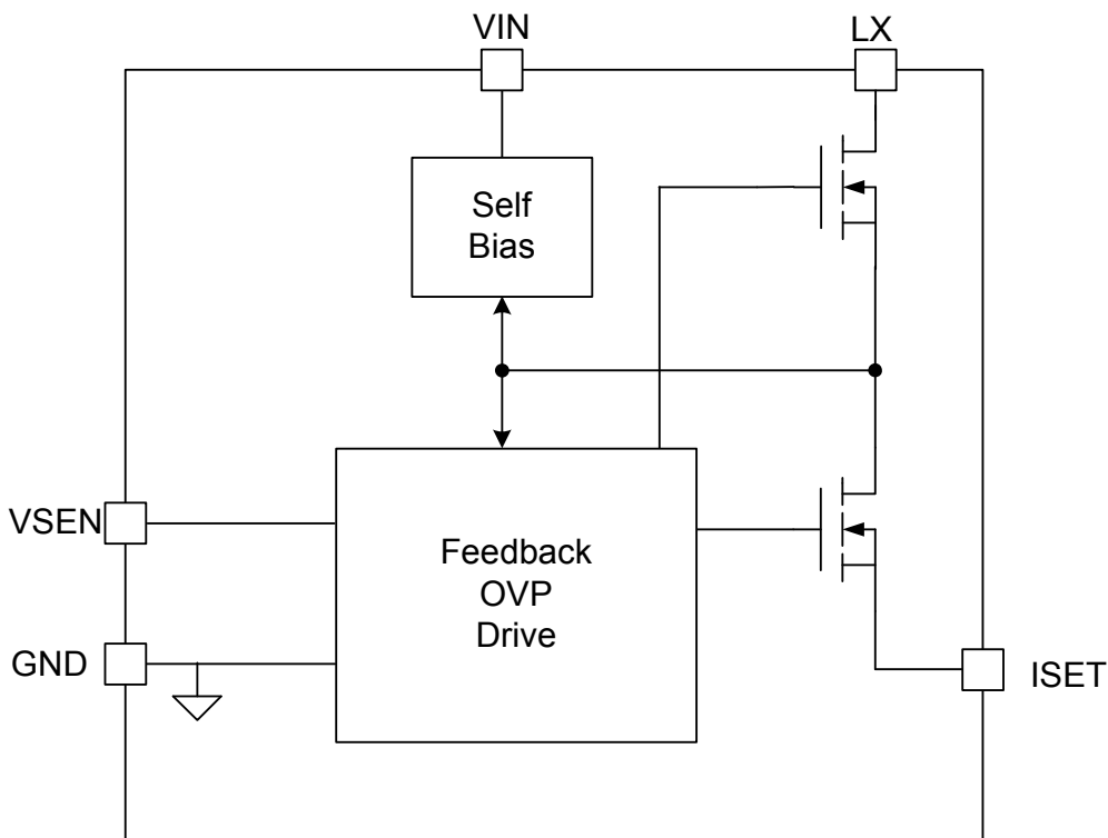
Figure2. Block Diagram
