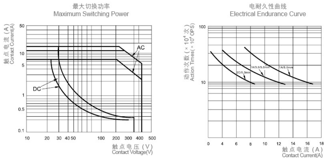
性能曲线图 PERFORMANCE CURVE
