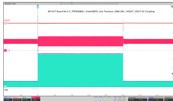
Figure 16. Line Transient
