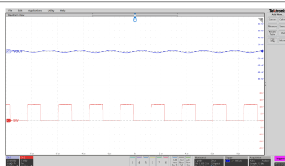
Figure 14. Output Voltage Ripple
