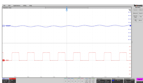
Figure 15. Output Voltage Ripple
