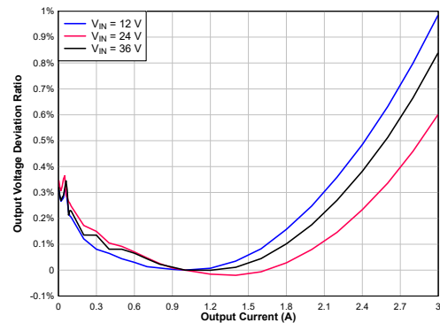
Figure 10. Line Regulation
