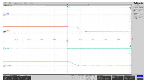
Figure 22. Power-Down by EN
