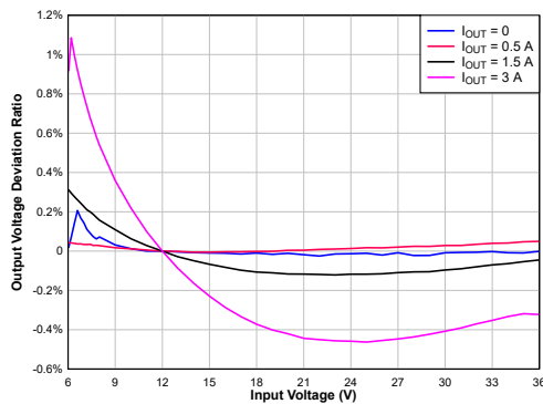
Figure 9. Load Regulation
