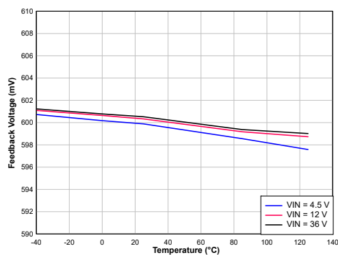
Figure 2. Reference Voltage vs. Junction Temperature
