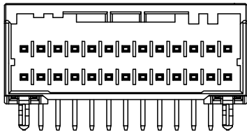
26POS: 560SBG-001H****T000
