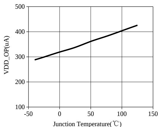
(c) V_{DD\_OP} VS T_J
