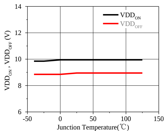
(b) V_{DD\_ON} , V_{DD\_OFF} VS T_J
