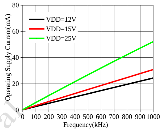
(j) VDD Current VS Frequency
